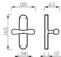
57 C CREMONESE WINDOW HANDLE
