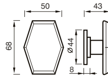
POMOLO C/ROSETTA KNOB W/ROSE
