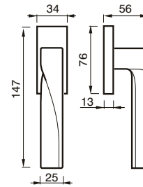
CREMONESE DK WINDOW HANDLE DK
