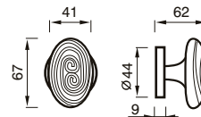
POMOLO C/ROSETTA KNOB W/ROSE
