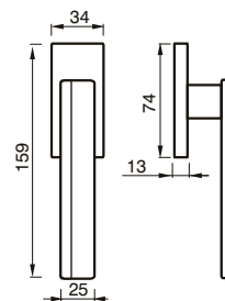
69 DK CREMONESE DK WINDOW HANDLE DK
