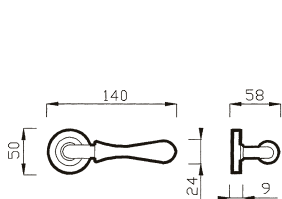
57 R MANIGLIA C/ROSETTA C/MOLLA HANDLE W/ROSE W/SPRING
