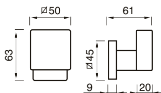
POMOLO C/ROSETTA C/MOLLA KNOB W/ROSE W/SPRING
